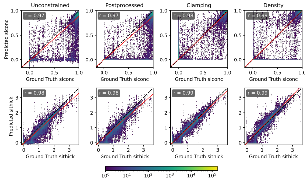
Predicted vs. true SIC and SIT at 30-day lead (1° ablation). The density channel (right) gives the most physical fields.
