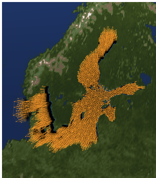
Baltic Sea hierarchy
